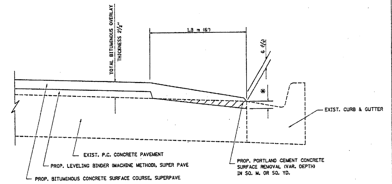
BITUMINOUS TAPER AT EDGE OF P.C.C. PAVEMENT
