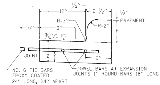
TYPE B-V.12 OR TYPE 3 CURB & GUTTER
