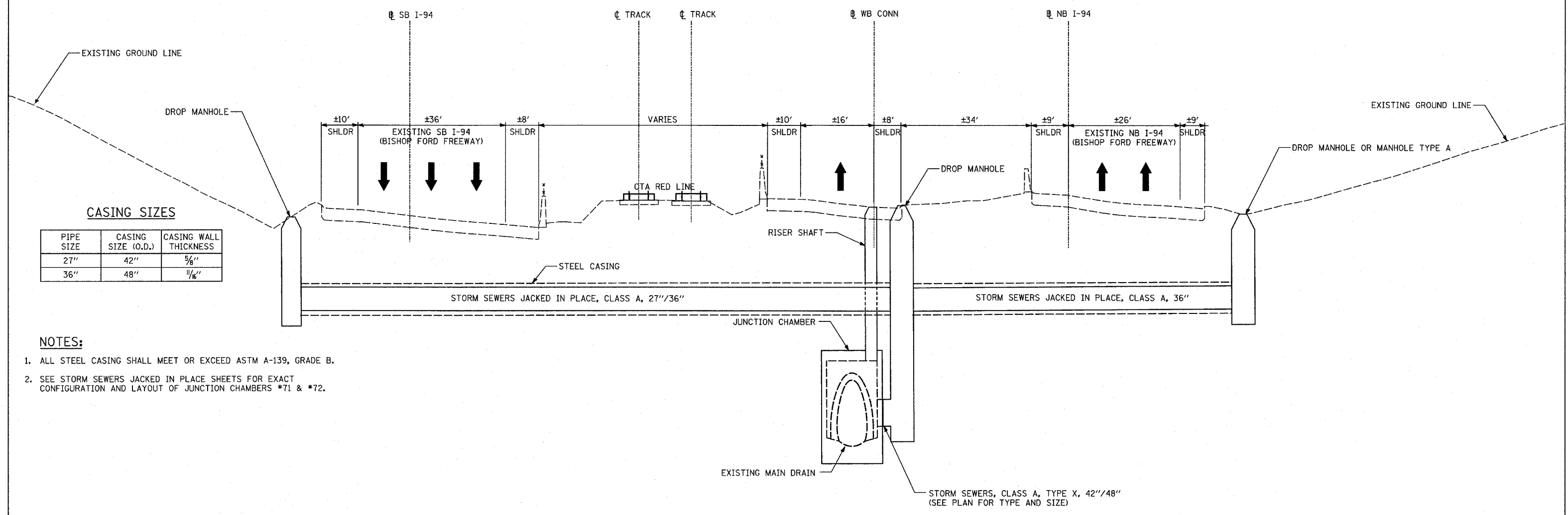
TYPICAL SECTION WITH STEEL CASING - 27" & 36" JACKED PIPE
