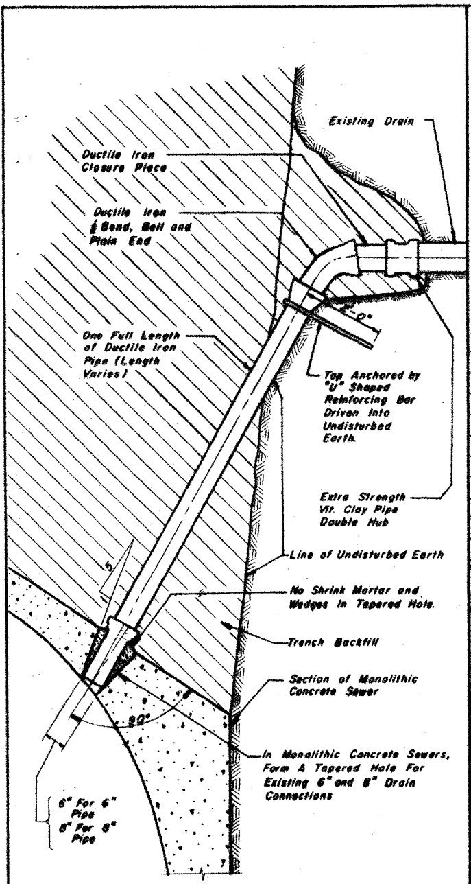
ELEVATION TYPICAL DRAIN CONNECTIONS FOR EXISTING DRAINS Items 76 and 7H
