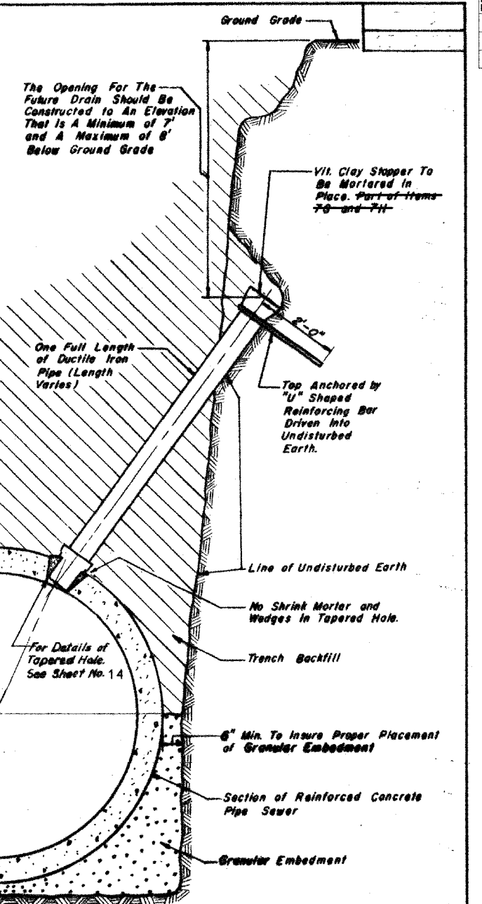
ELEVATION TYPICAL DRAIN STACKS FOR FUTURE USE Items 76 and 7H
