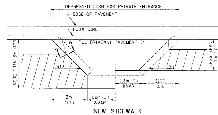
NEW SIDEWALK
