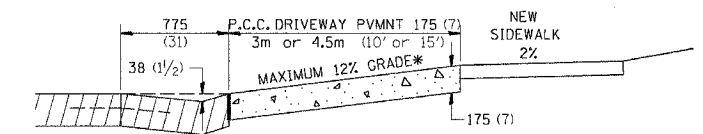
ASCENDING APPROACH
