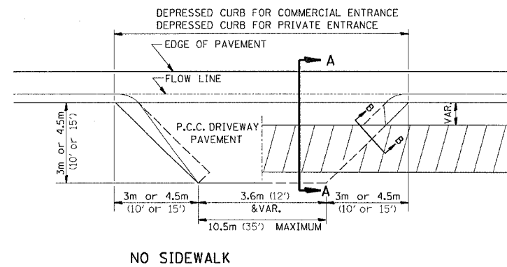
NO SIDEWALK
