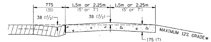
DESCENDING APPROACH
