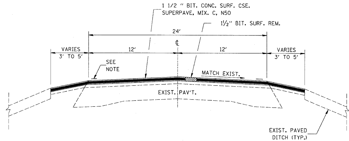
TYPICAL SECTION STA. 104+10 TO STA. 111+40 NOTE: ROAD WILL BE STRIPED FOR 22' (TYP.)
