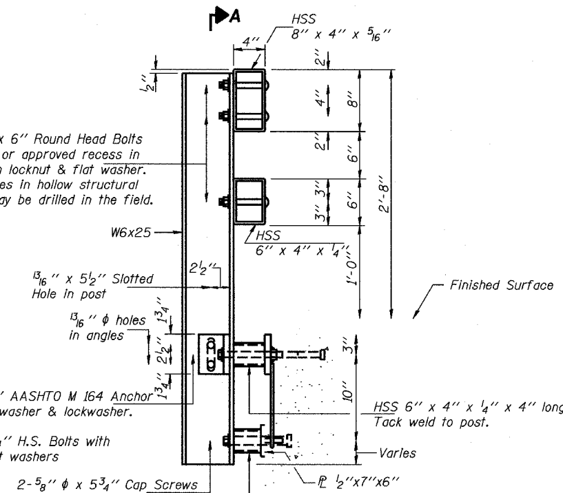
RAIL SPLICE CONNECTION AT EXPANSION JT.
