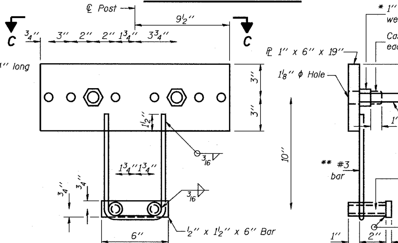
SECTION AT RAIL POST
