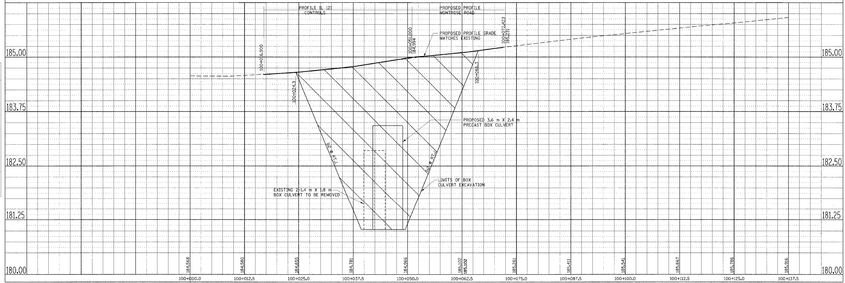
PROFILE, MONTROSE ROAD, CUMBERLAND CO. STA. 100+000.0 TO STA. 100+137.5, (FAP 828) MONTROSE RD.
