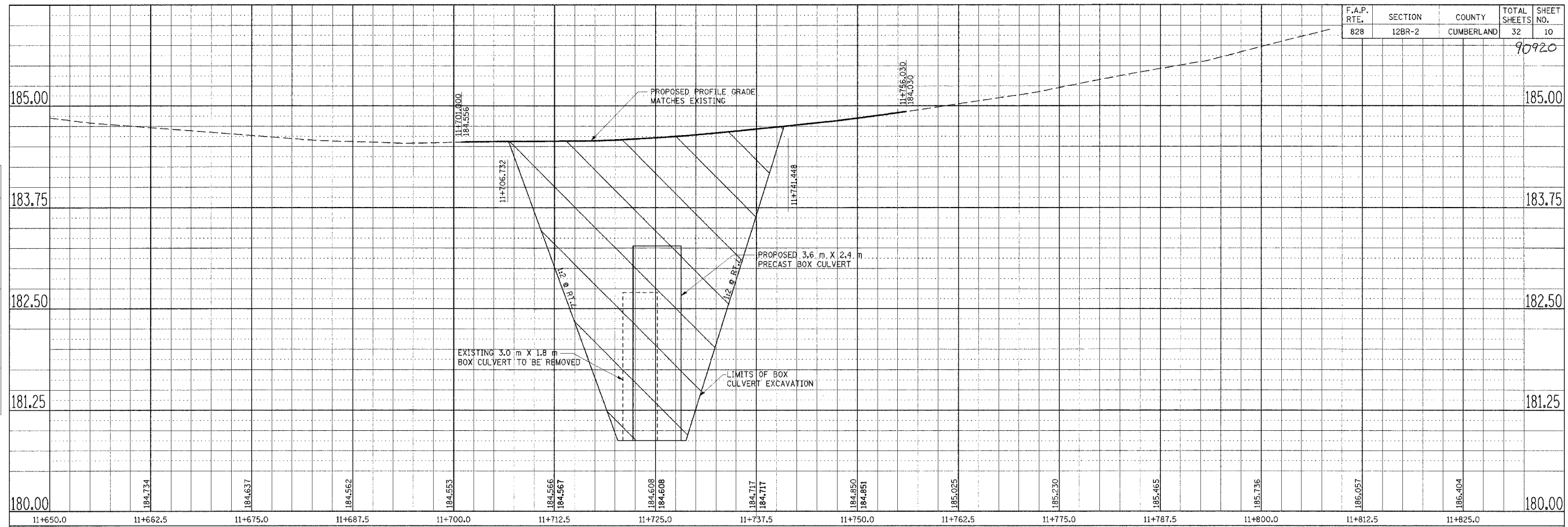
PROFILE, ILLINOIS ROUTE 121, CUMBERLAND CO. STA. 11+650.0 TO STA. 11+825.0
