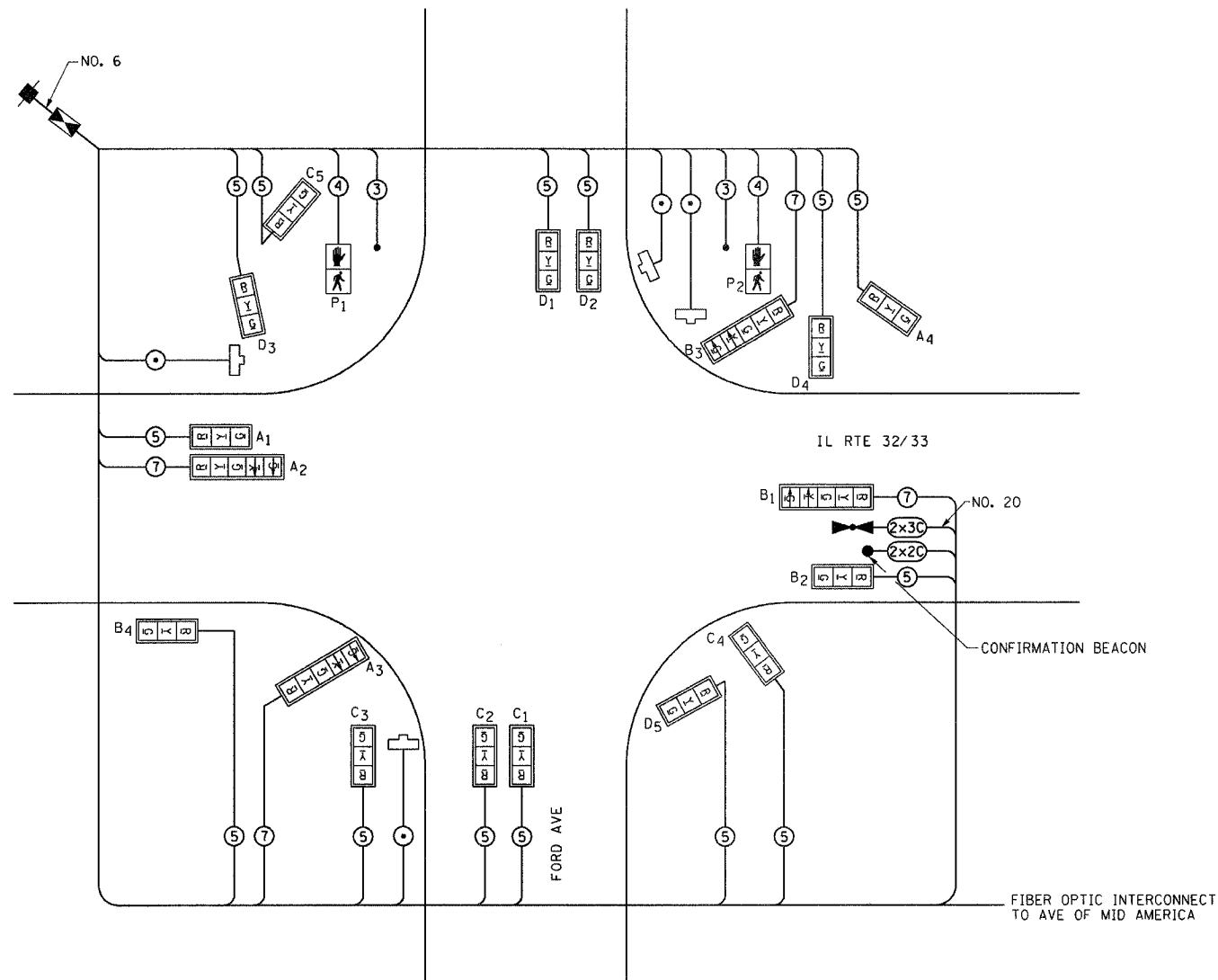
TRAFFIC SIGNAL SCHEMATIC
