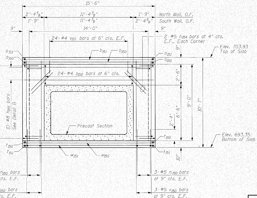
NORTH WALL ELEVATION SOUTH WALL ELEVATION
