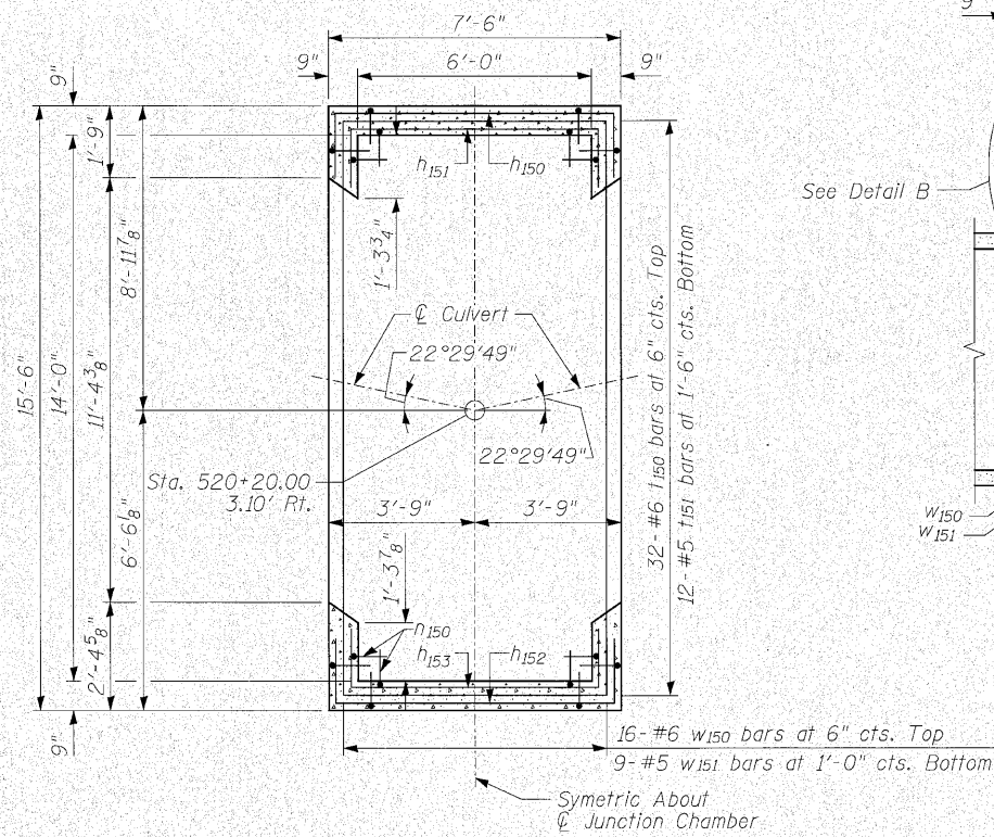
BOTTOM SLAB PLAN
