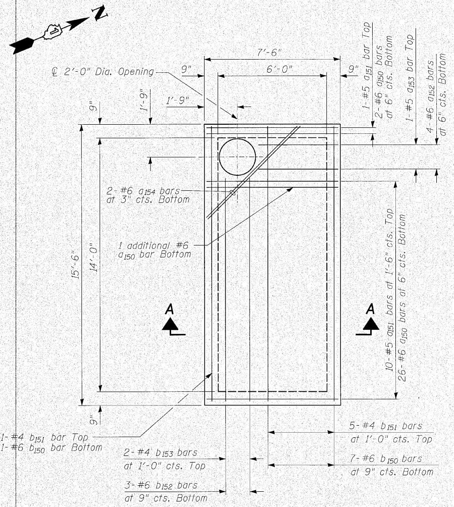
TOP SLAB PLAN
