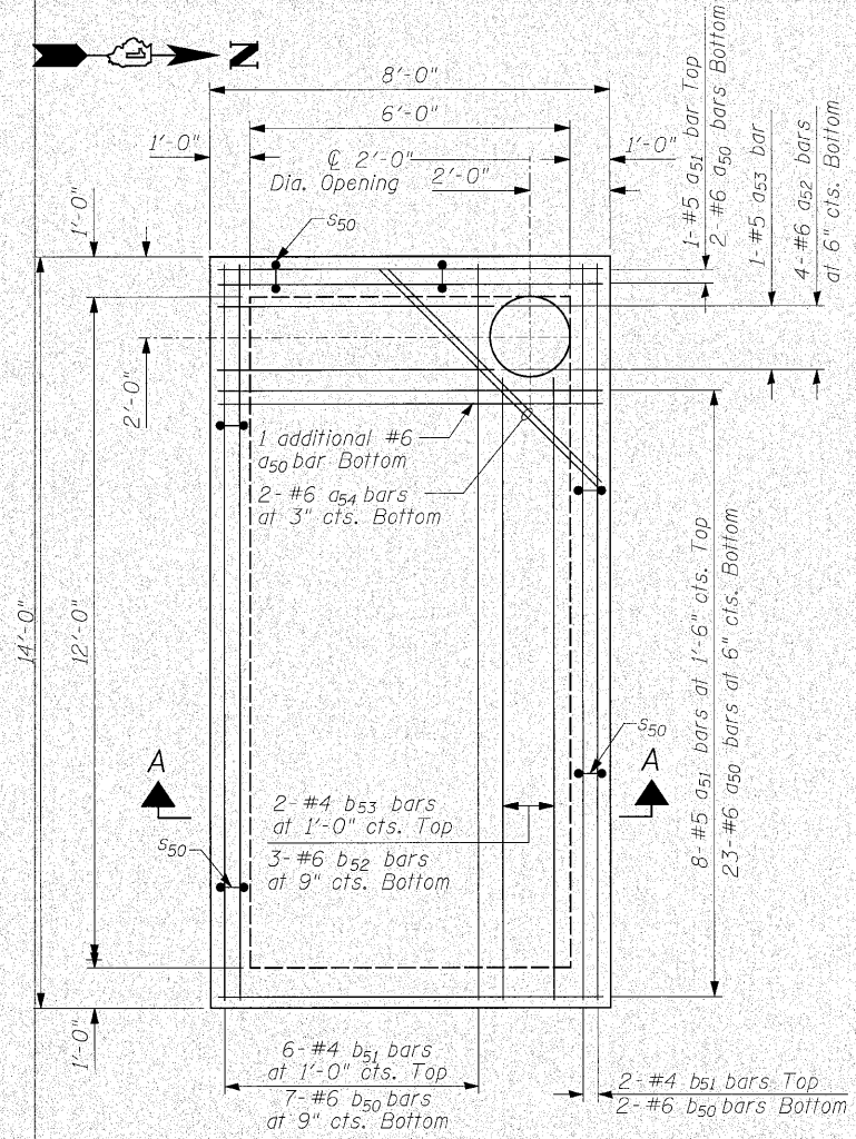
TOP SLAB PLAN
