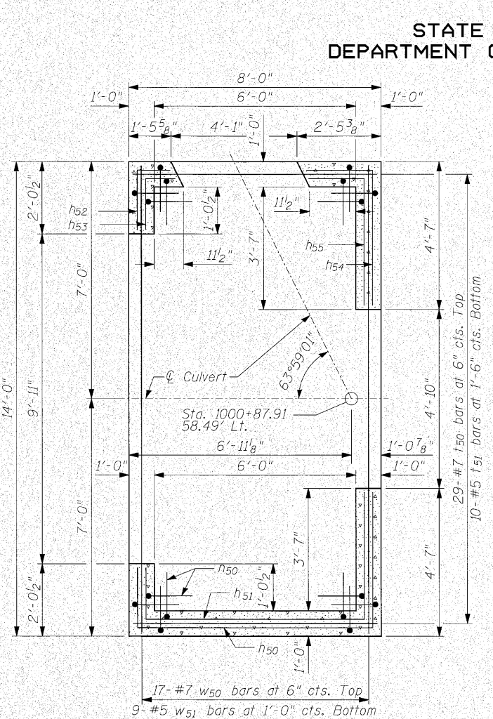
BOTTOM SLAB PLAN
