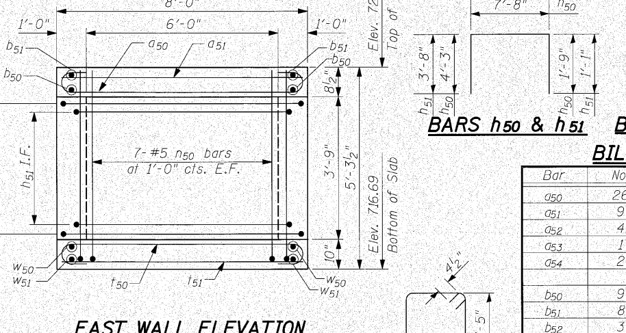
EAST WALL ELEVATION
