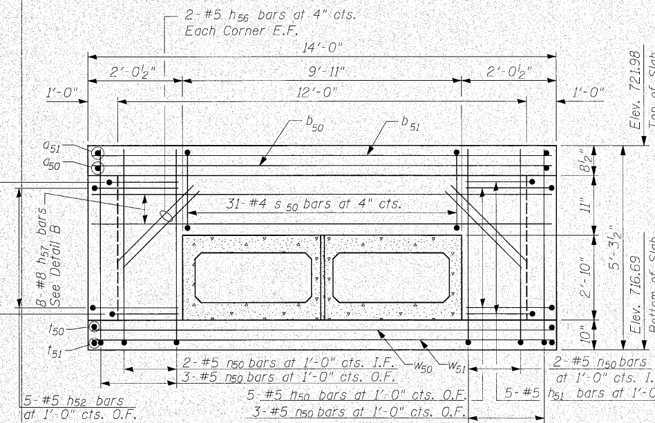
SOUTH WALL ELEVATION
