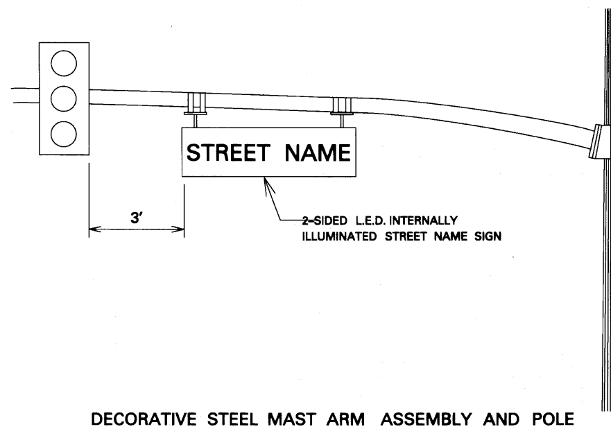
DECORATIVE STEEL MAST ARM ASSEMBLY AND POLE
