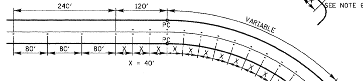
TYPICAL RAISED PAVEMENT MARKER INSTALLATION
