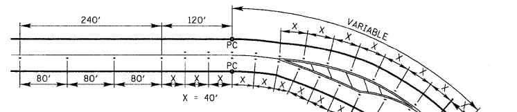
TYPICAL RAISED PAVEMENT MARKER INSTALLATION
