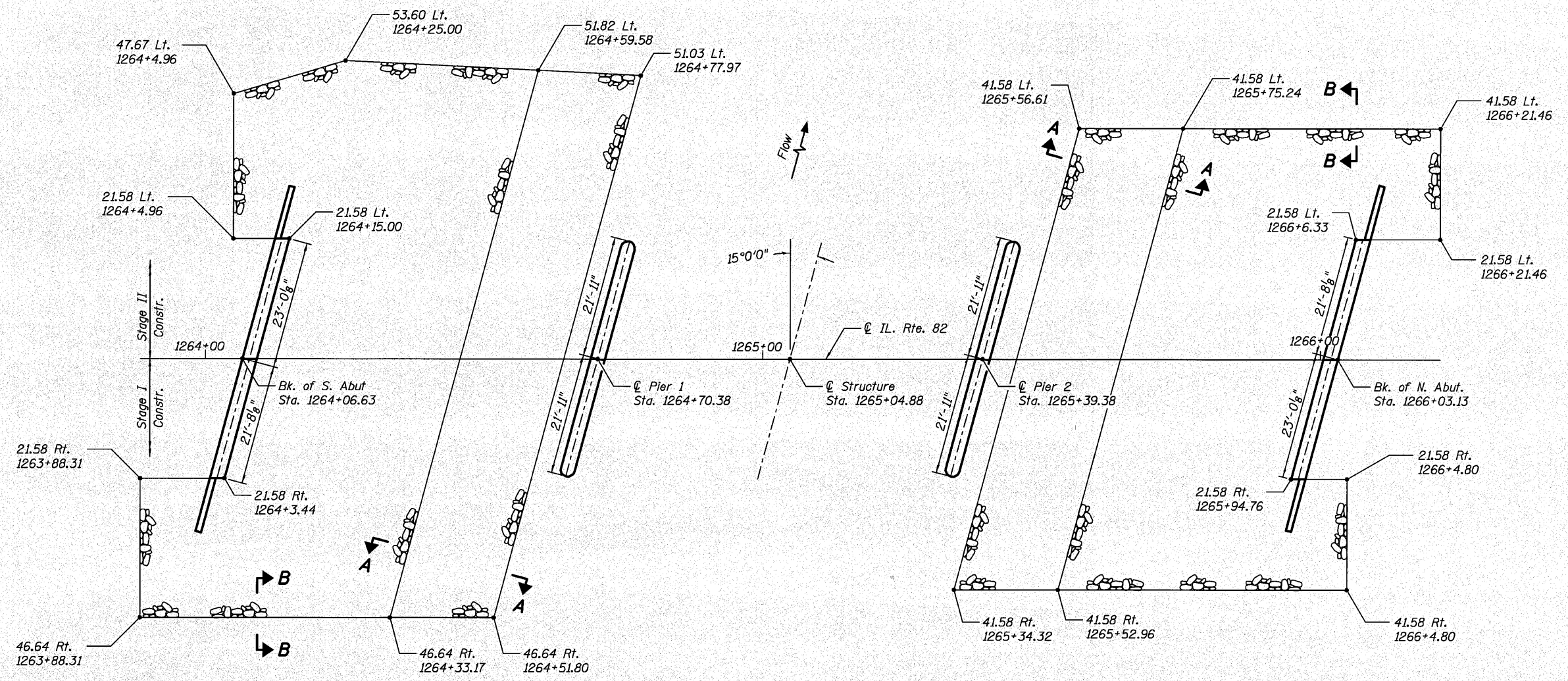
FOOTING AND RIPRAP LAYOUT
