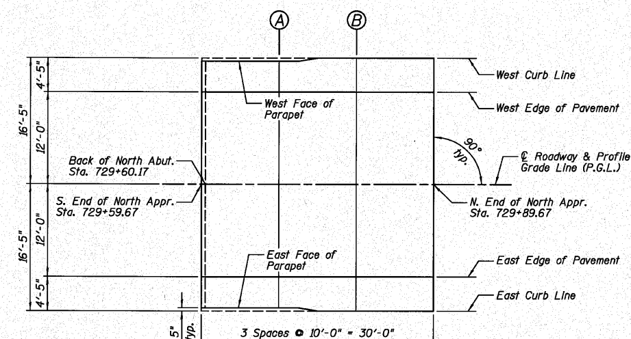
NORTH APPROACH SLAB PLAN
