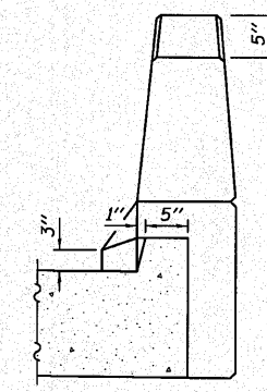
VIEW B-B
