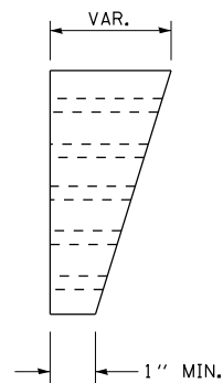
PARAPET WOOD BLOCK-OUT DETAIL
