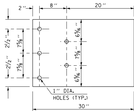
PARAPET WOOD BLOCK-OUT DETAIL
