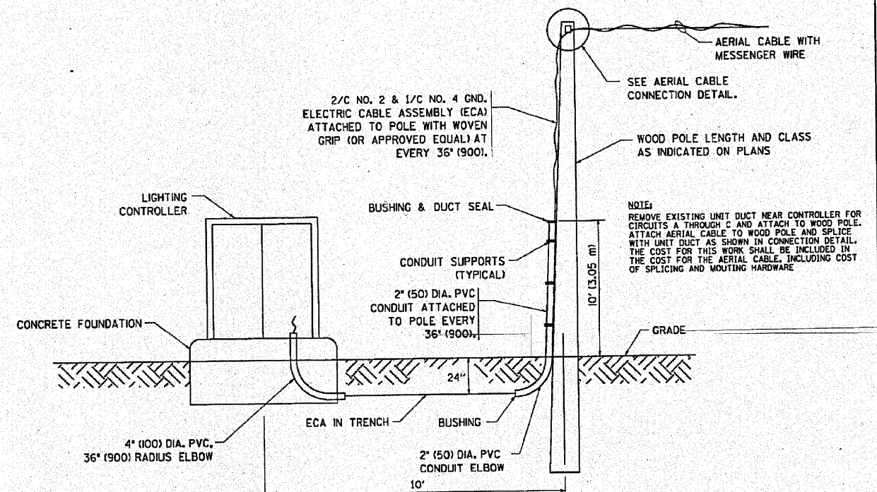
WOOD POLE TO LIGHTING CONTROLLER WIRING CONNECTION DETAIL N.T.S.
