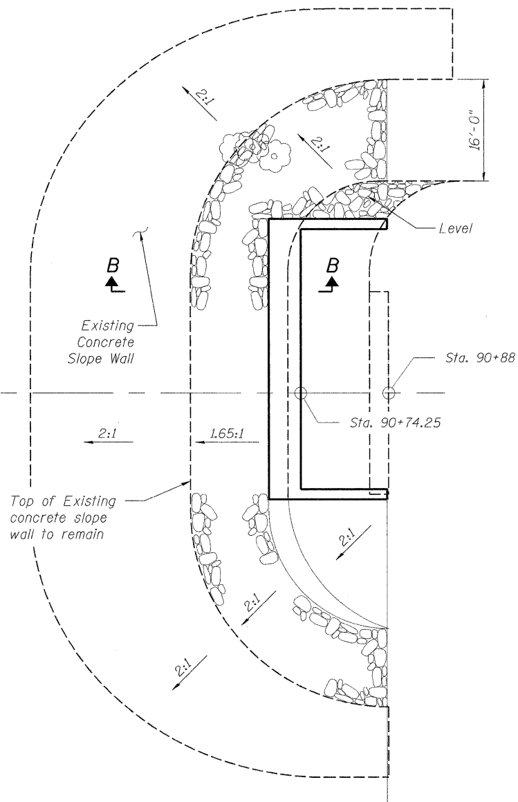
WEST SLOPE PROTECTION PLAN
