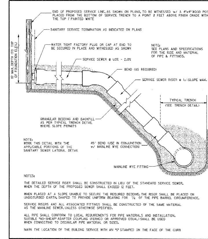
DeKalb Sanitary District 303 Hollister Avenue • DeKalb, Illinois 60115 815.758.3313 Fax: 815.758.6615 DETAIL No. 14 Sanitary Sewer Service Riser Detail DATE: 06/12/07 REV: 4
