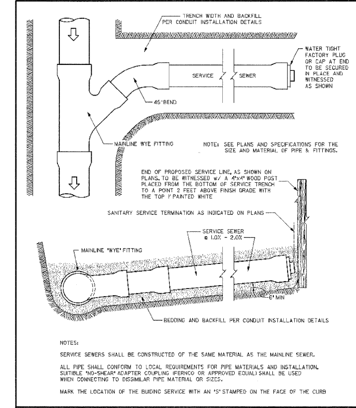
DeKalb Sanitary District 303 Hollister Avenue • DeKalb, Illinois 60115 815.758.3313 Fax: 815.758.6615 DETAIL No. 13 Sanitary Sewer Service Lateral Detail DATE: 06/12/07 REV: 4
