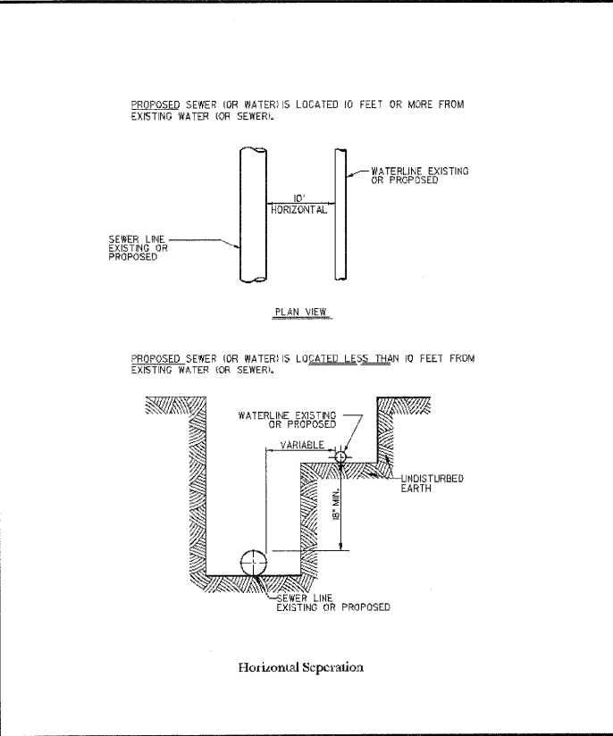
DeKalb Sanitary District 303 Hollister Avenue • DeKalb, Illinois 60115 815.758.3313 Fax: 815.758.6615 DETAIL No. 11 Horizontal Water and Sewer Separation Requirement - Detail DATE: 06/12/07 REV: 4
