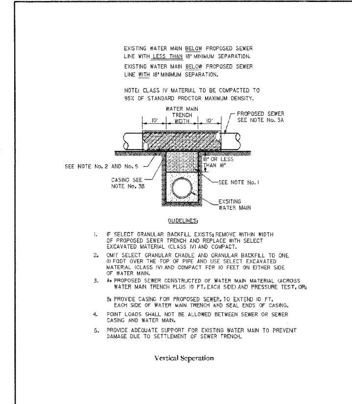
DeKalb Sanitary District 303 Hollister Avenue • DeKalb, Illinois 60115 815.758.3313 Fax: 815.758.6615 DETAIL No. 10 Water and Sewer Separation Requirement - Detail DATE: 06/12/07 REV: 4
