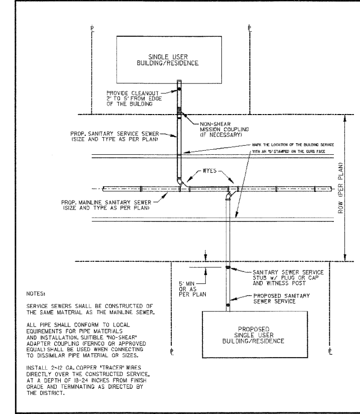
DeKalb Sanitary District 303 Hollister Avenue • DeKalb, Illinois 60115 815.758.3313 Fax: 815.758.6615 DETAIL No. 12 Sanitary Sewer Service Detail DATE: 06/12/07 REV: 4
