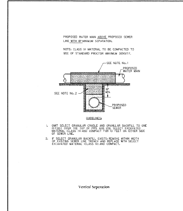
DeKalb Sanitary District 303 Hollister Avenue • DeKalb, Illinois 60115 815.758.3313 Fax: 815.758.6615 DETAIL No. 8 Water and Sewer Separation Requirement - Detail DATE: 06/12/07 REV: 4
