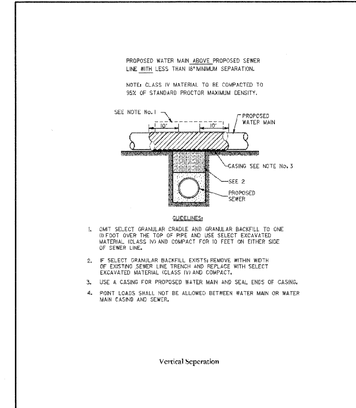
DeKalb Sanitary District 303 Hollister Avenue • DeKalb, Illinois 60115 815.758.3313 Fax: 815.758.6615 DETAIL No. 9 Water and Sewer Separation Requirement - Detail DATE: 06/12/07 REV: 4
