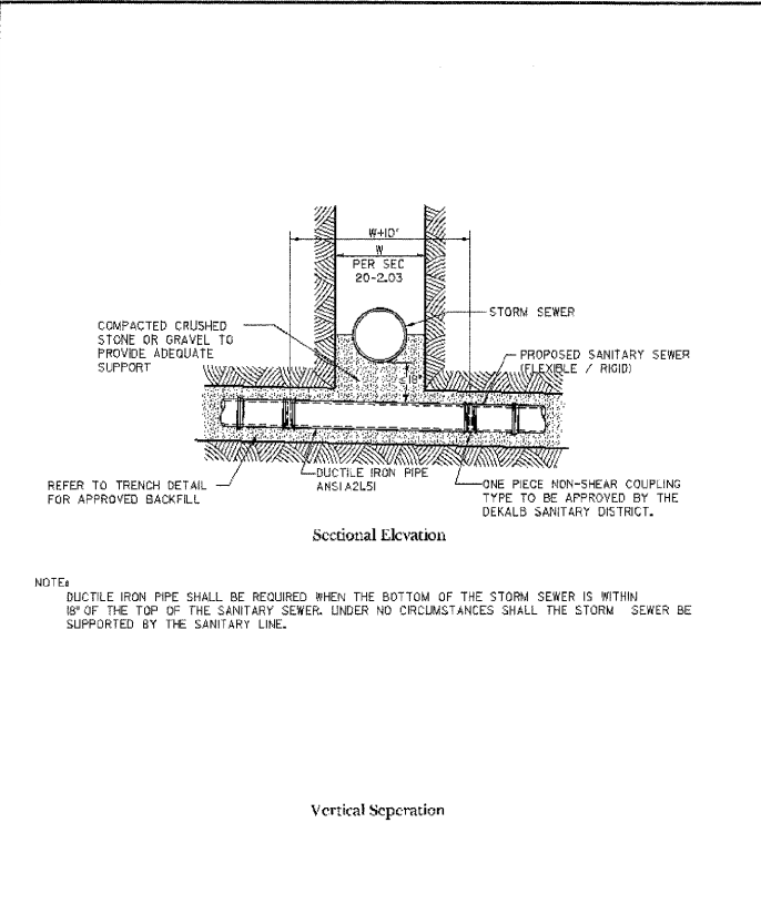
DeKalb Sanitary District 303 Hollister Avenue • DeKalb, Illinois 60115 815.758.3313 Fax: 815.758.6615 DETAIL No. 7 Sanitary Sewer at Storm Sewer Crossing Detail DATE: 06/12/07 REV: 4
