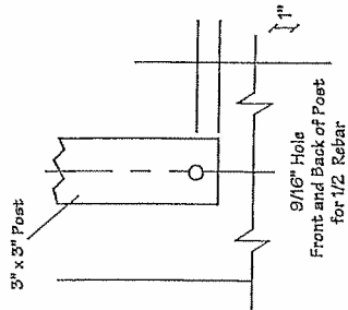
2 Underground Portion of Post
