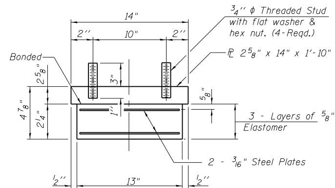
BEARING ASSEMBLY
