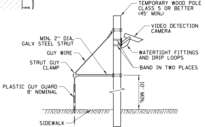
TEMPORARY POLE DETAIL WITH SIDEWALK STRUT AND TYP. VIDEO DETECTION MOUNTING (NOT TO SCALE)
