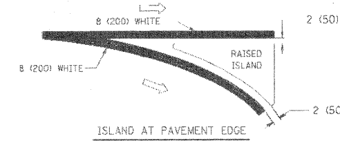
ISLAND OFFSET FROM PAVEMENT EDGE
