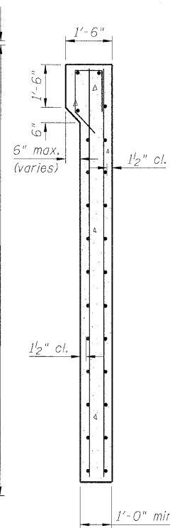
SECTION THRU PANEL
