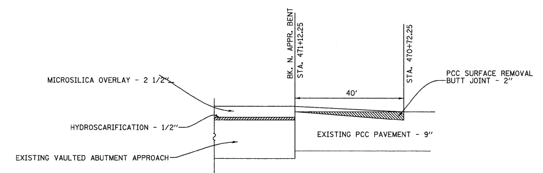
BUTT JOINT DETAIL
