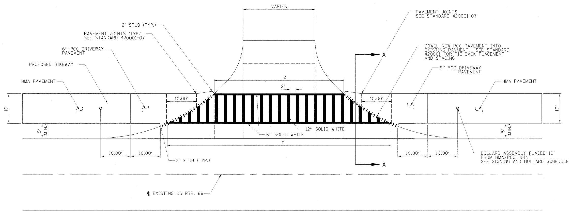
TYPICAL CONCRETE ENTRANCE DETAIL
