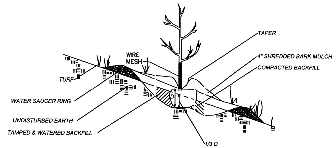
HILLSIDE PLANTING DEPTH
