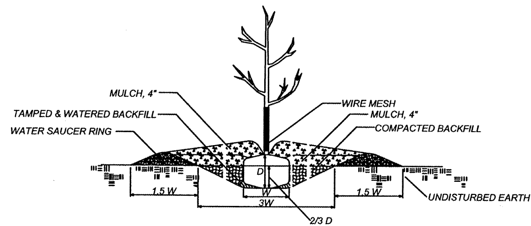
FLAT GROUND PLANTING DETAIL
