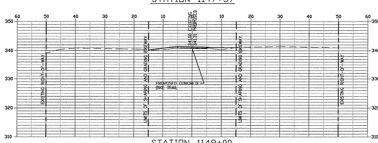
STATION 1149+00
