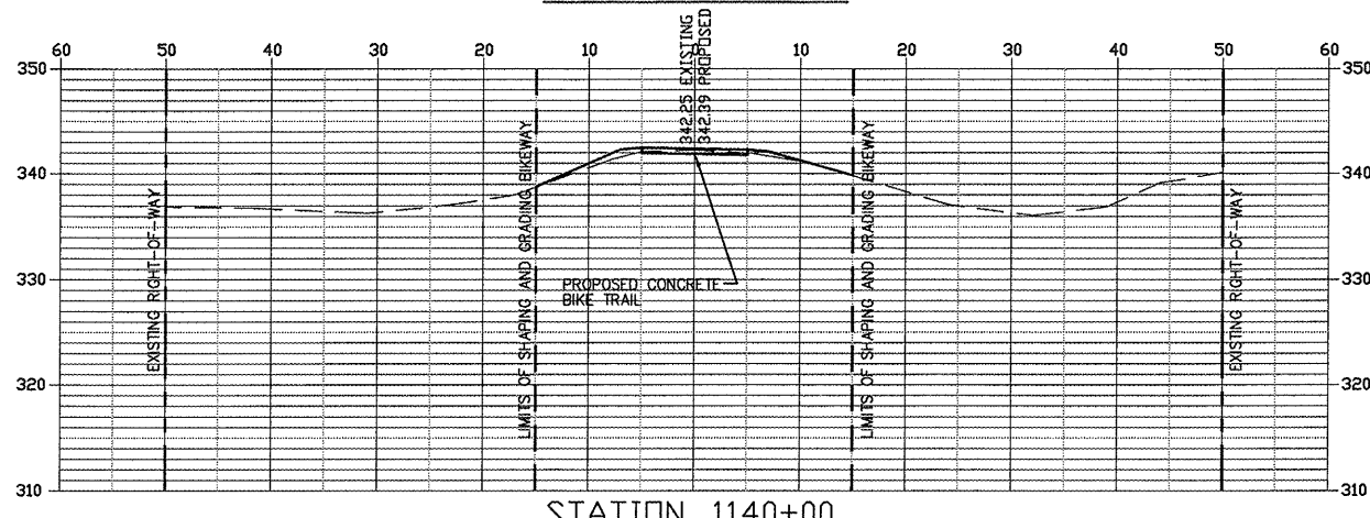
STATION 1140+00
