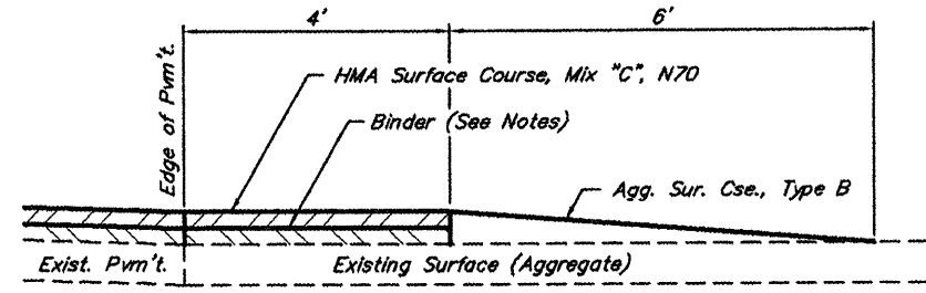
SECTION A-A PRIVATE ENTRANCE - AGGREGATE (Est. No. = 39)
