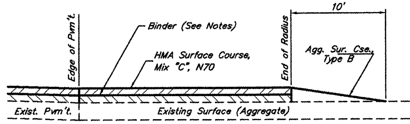
SECTION A-A SIDE ROAD - AGGREGATE (Est. No. = 0)
