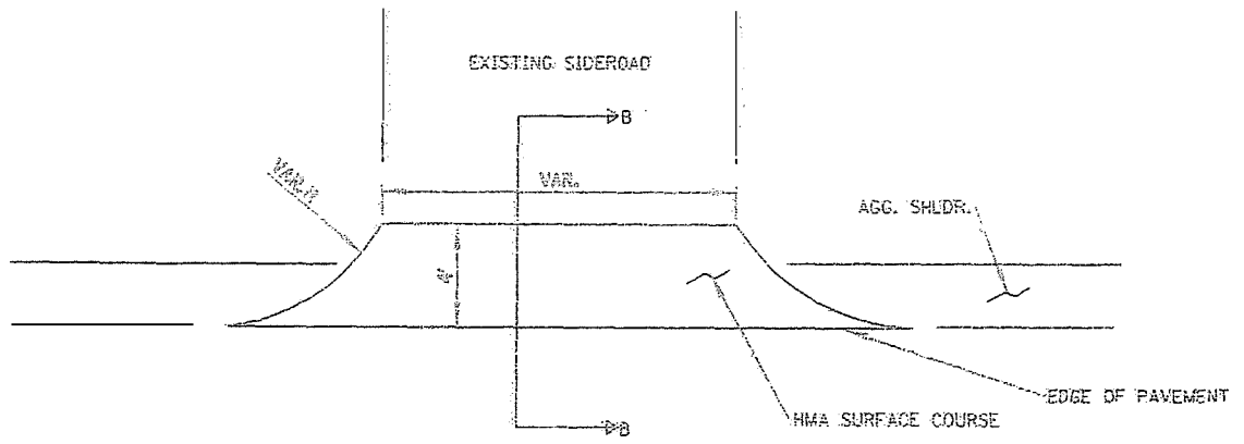
SIDEROAD DETAIL
