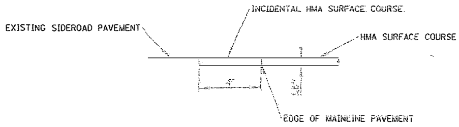
SECTION B-B
