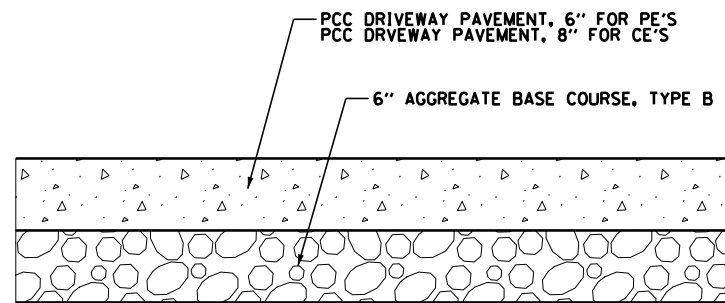
PCC DRIVEWAY PAVEMENT SECTION
