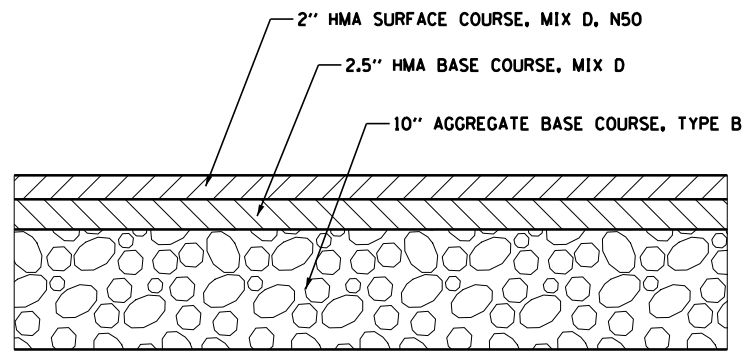
HMA DRIVEWAY PAVEMENT SECTION
