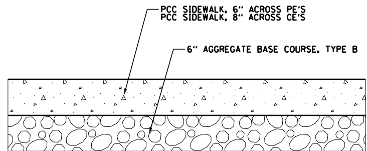
PCC SIDEWALK SECTION ACROSS DRIVEWAYS
