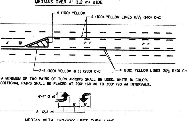
TYPICAL PAINTED MEDIAN MARKING
