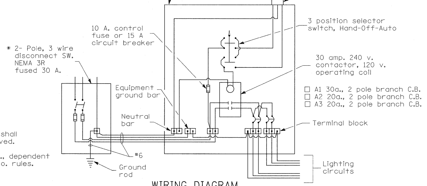
WIRING DIAGRAM
