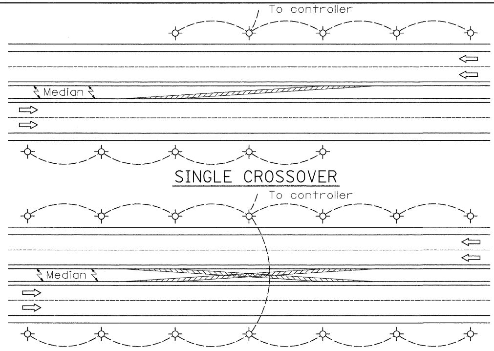
DUAL CROSSOVER
