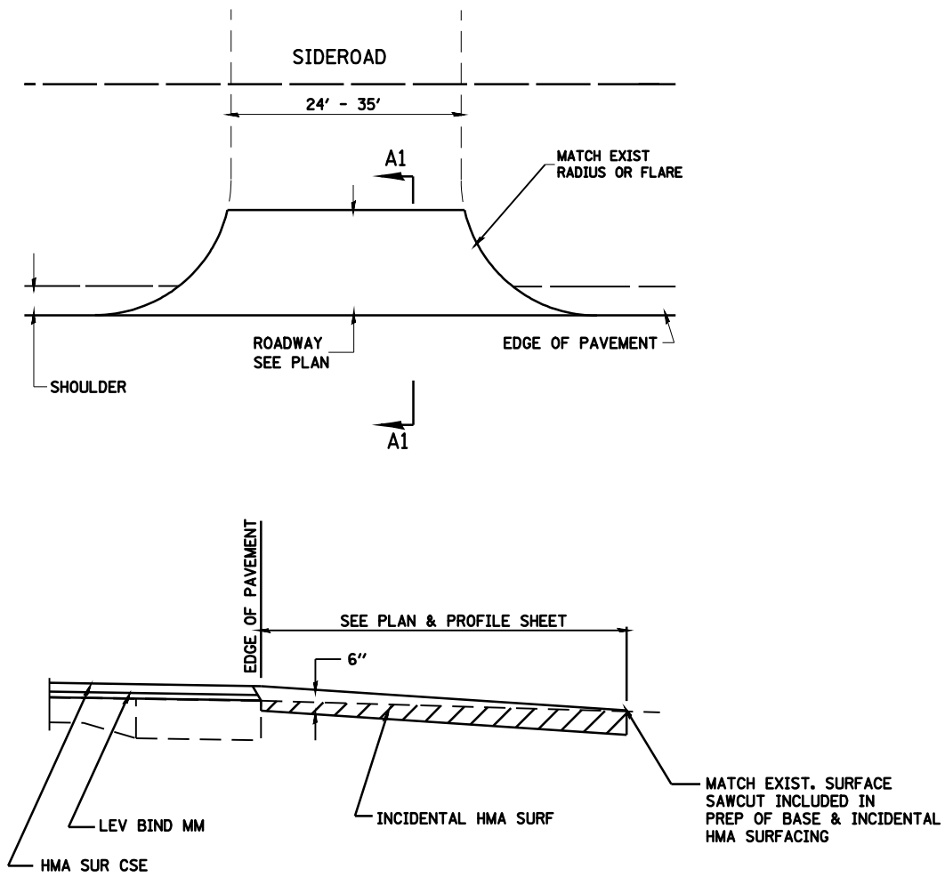
SECTION A1-A1 FOR SIDEROAD
