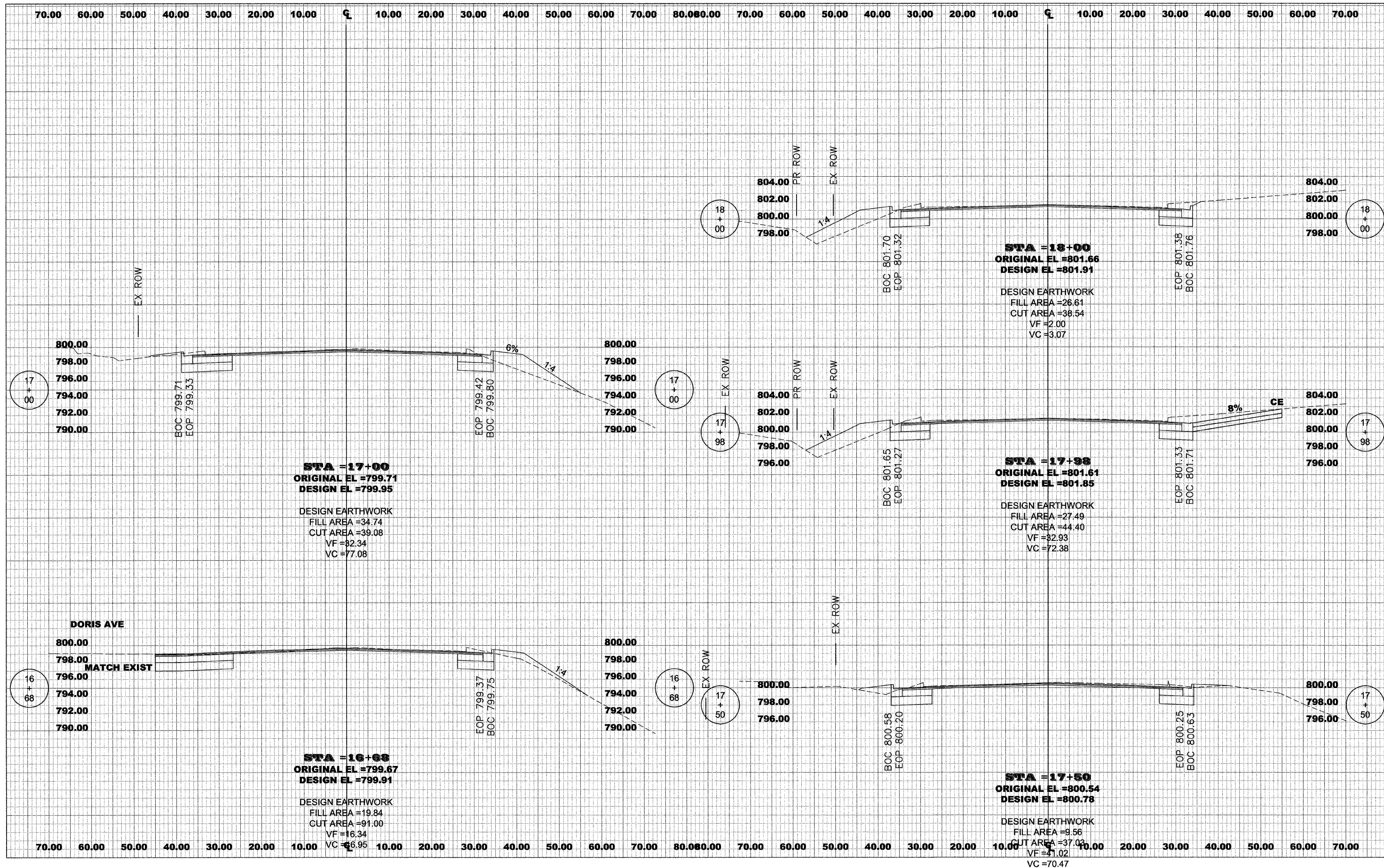
SPRINGFIELD AVE CROSS-SECTION
