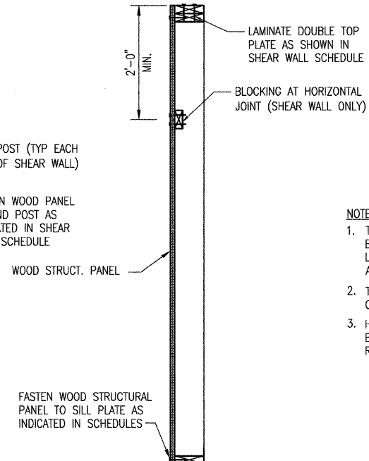
TYP. EXT. WALL SECTION FOR SHEAR & NONSHEAR WALLS
