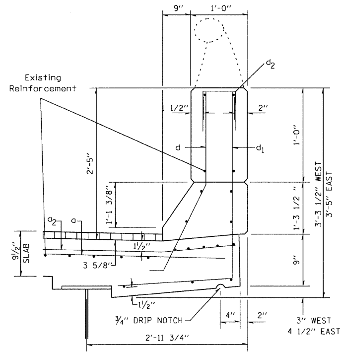
PARAPET DETAIL
