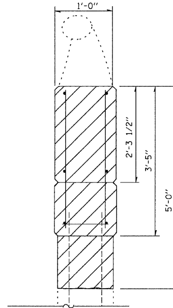
WINGWALL DETAIL
