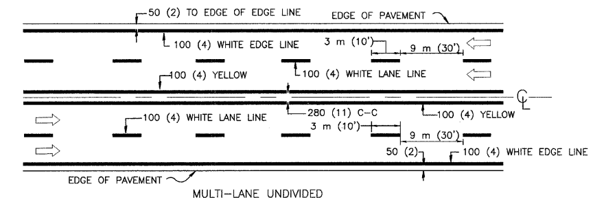
MULTI-LANE UNDIVIDED
