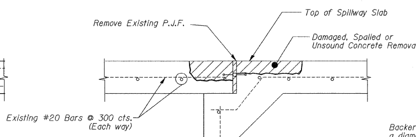
TYPE III EXISTING JOINT (Repair Concrete Structures)
