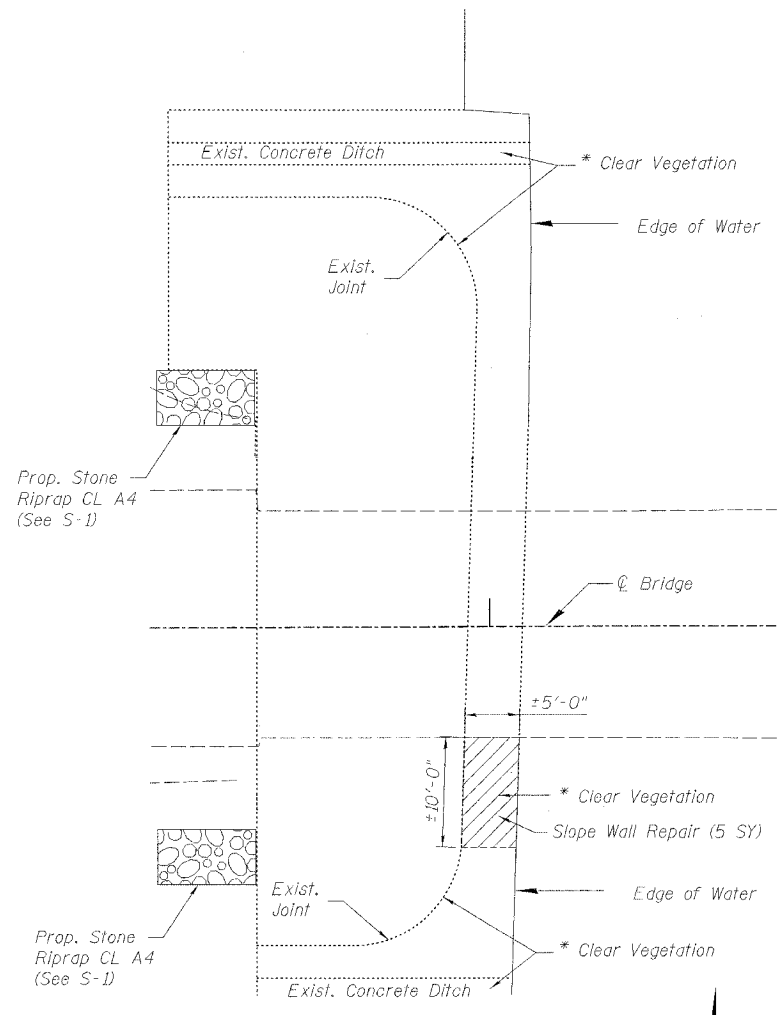
WEST SLOPEWALL REPAIR PLAN
