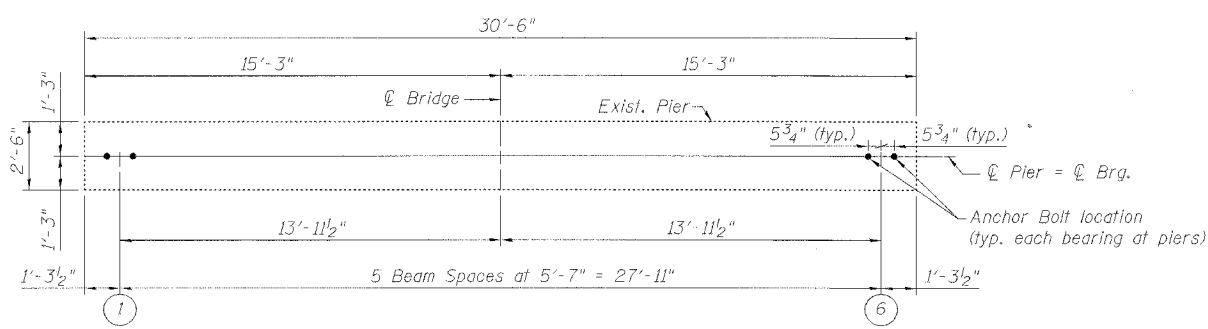
PIER ANCHOR BOLT LOCATION PLAN
