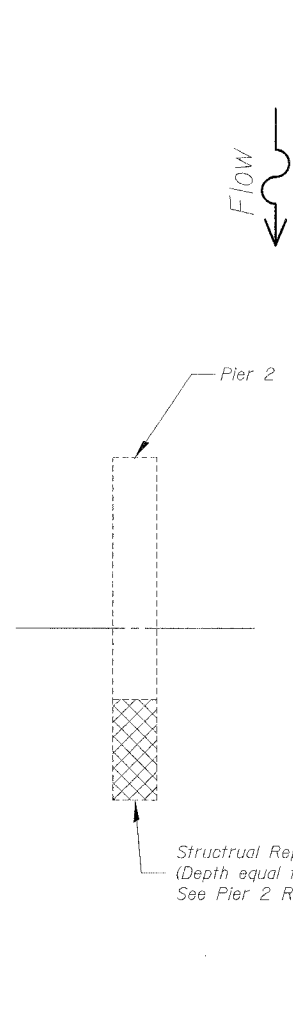
PIER 2 REPAIR PLAN
