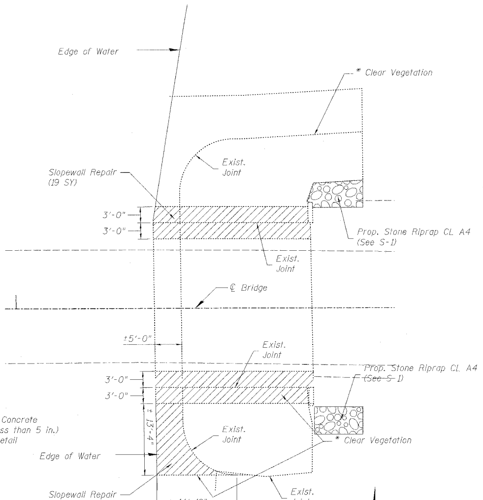
EAST SLOPEWALL REPAIR PLAN
