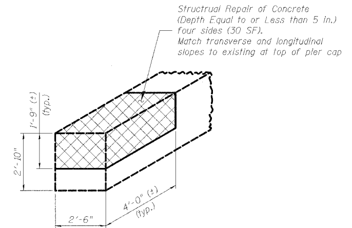
PIER 2 REPAIR DETAIL
