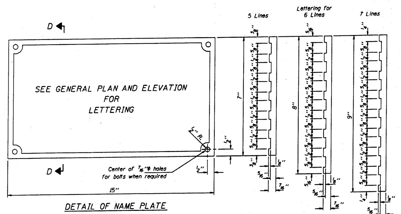
SECTIONS D-D
