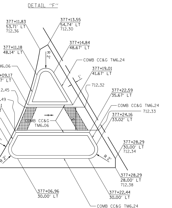
DETAIL - CONCRETE MEDIAN (SPECIAL) (NOT TO SCALE)
