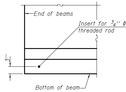
ELEVATION OF BEAM AT END
