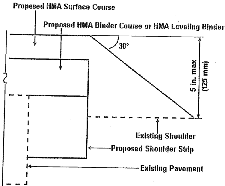
Safety Edge at Edge of Shoulder Strips
