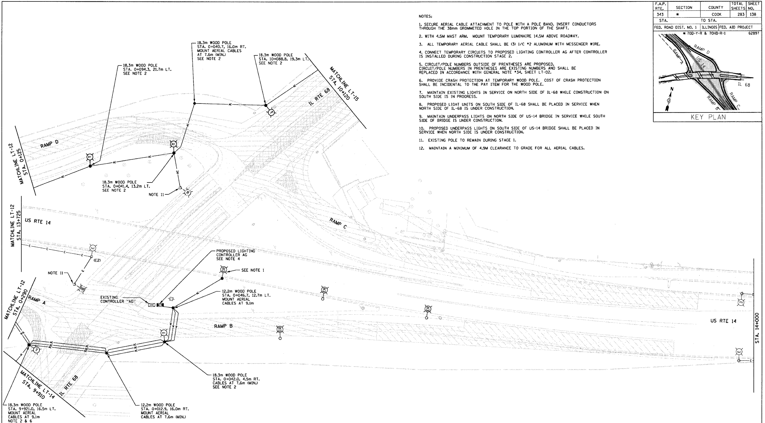
1 ROADWAY TEMPORARY LIGHTING PLAN SCALE: 1 : 500 5 0 5 10 15 20 25 SCALE IN METERS
