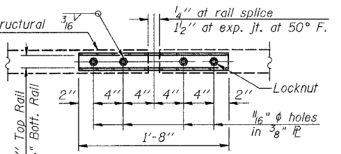
PLAN-BOTT. SPLICE TYPICAL
