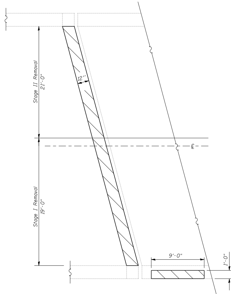
EXISTING PARTIAL PLAN Joint at South Abutment
