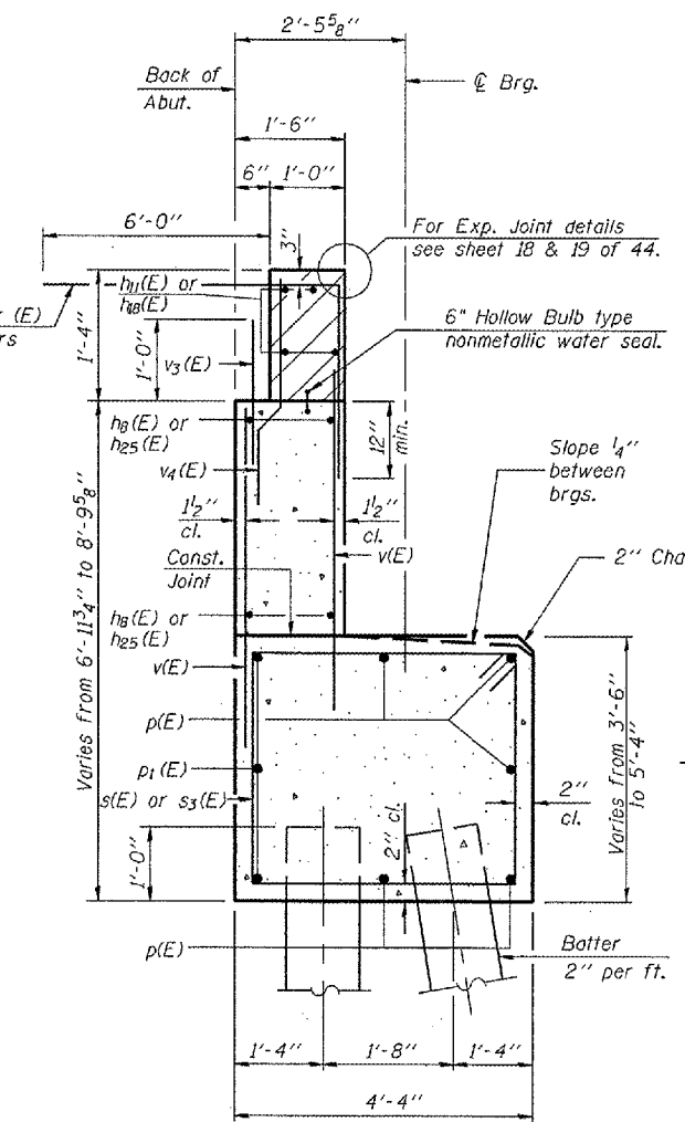
SEC. THRU ABUT.
