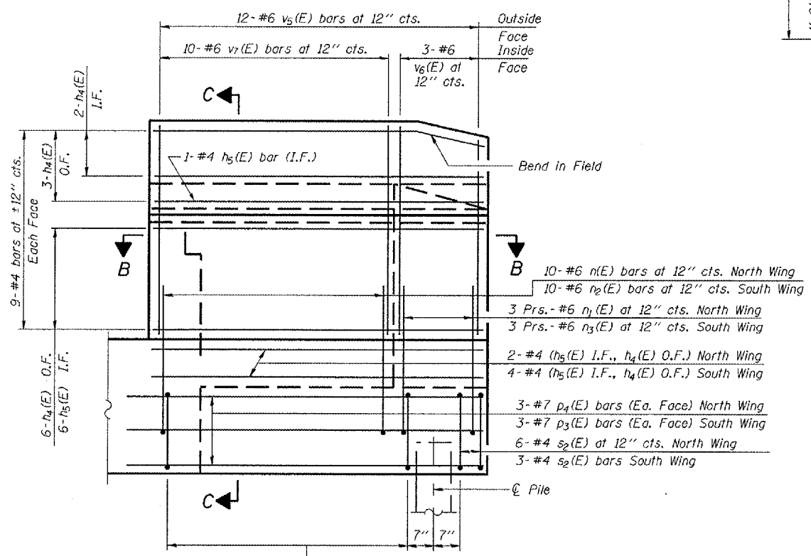
WING WALL ELEVATION Showing Reinforcement
