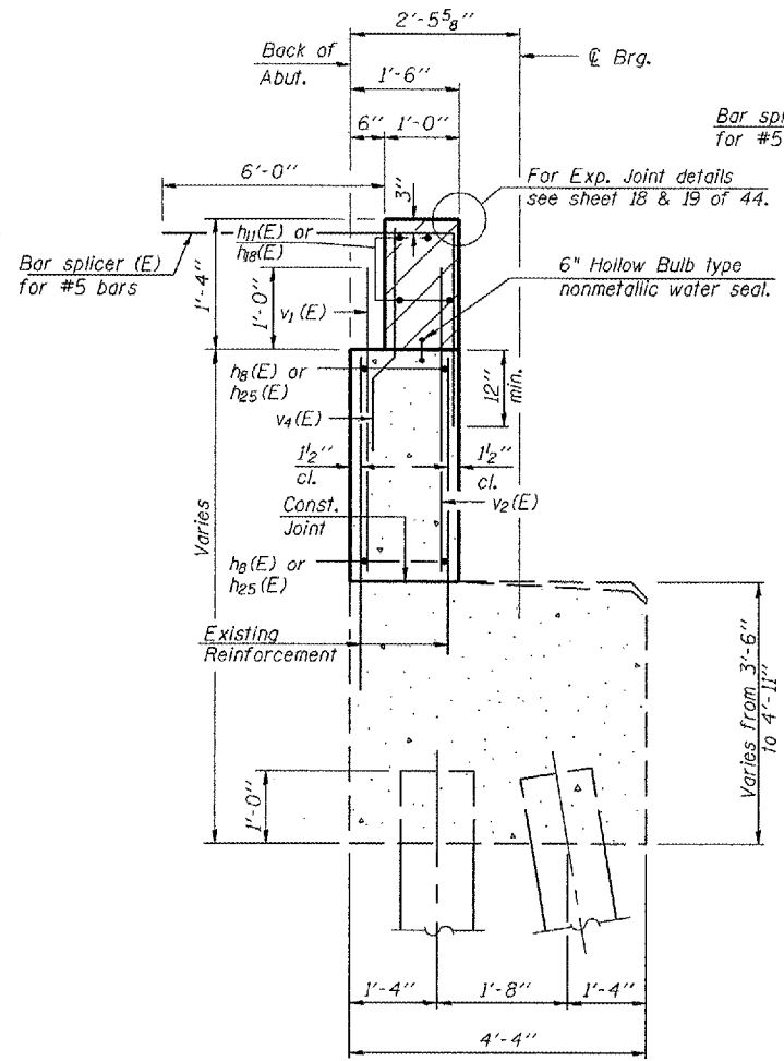
SEC. THRU EXISTING ABUT.
