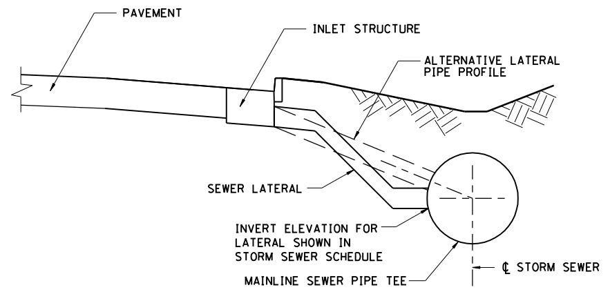
STORM SEWER LATERAL @ PIPE TEE NOT TO SCALE
