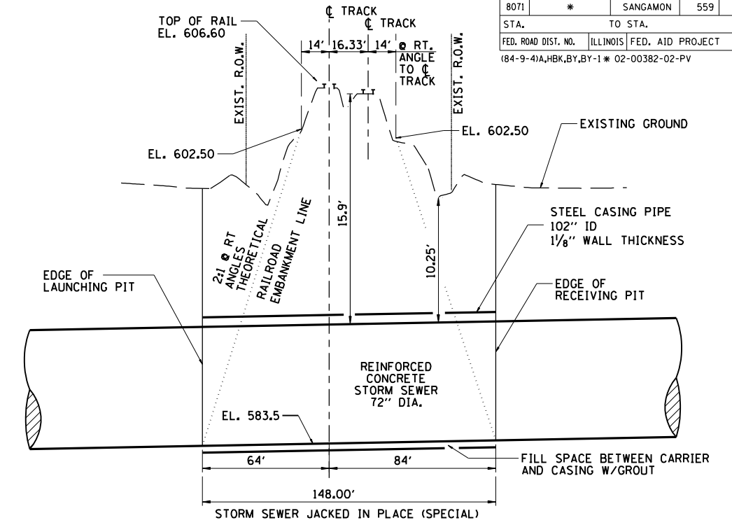
ELEVATION MACARTHUR BOULEVARD STORM SEWER BENEATH NORFOLK SOUTHERN RAILWAY NOT TO SCALE
